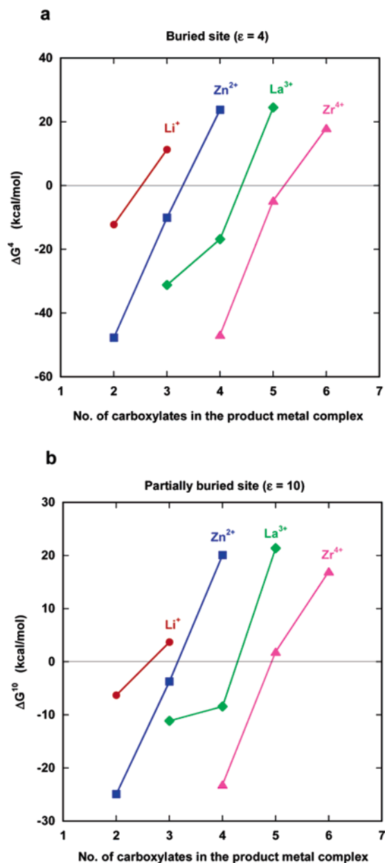
FIGURE 3. Calculated free energies ( \Delta G^\circ ) for the successive exchange of a metal-bound water molecule for monodentately bound acetate in [M(H_2O)_m(CH_3COO)_n]^{q-n} complexes ( M = Li^+, Zn^{2+}, La^{3+} , and Zr^{4+} ) as a function of the number of carboxylates in the product metal complex. (a) \Delta G^\circ corresponding to a buried site ( \epsilon = 4 ). (b) \Delta G^\circ corresponding to a partially buried site ( \epsilon = 10 ).
